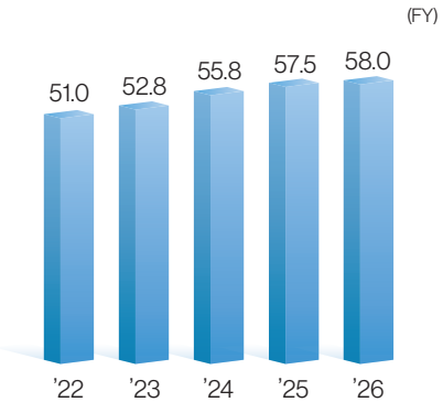
Engagement Score
